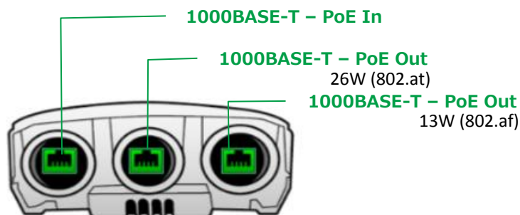
Terminal unit
